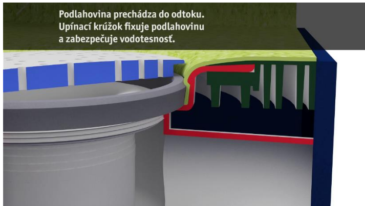
Clamping ring 130, automatic, 7141316
